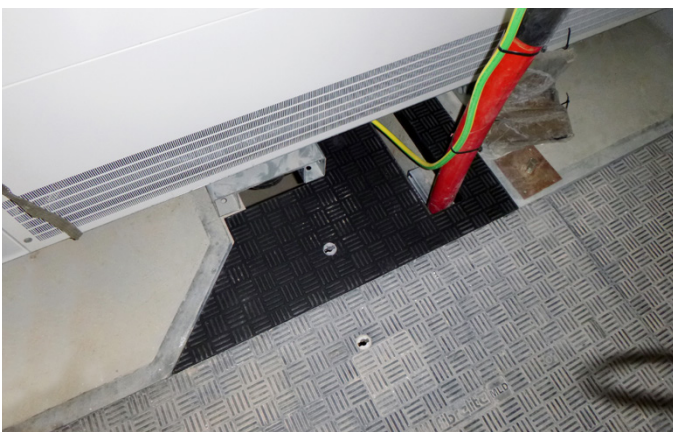
Custom Fibrelite trench access covers designed with cut-outs to accommodate piping and cabling
