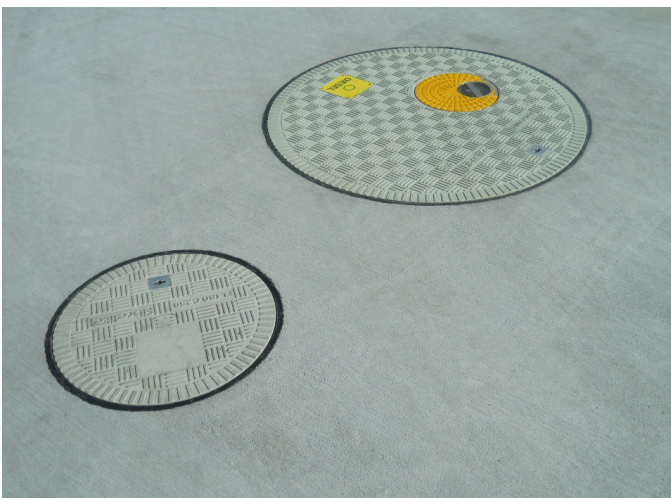
Fibrelite's offset fill port (8" off centre) with color coded easily removable, watertight fill ports together with an 18" watertight monitoring well cover
