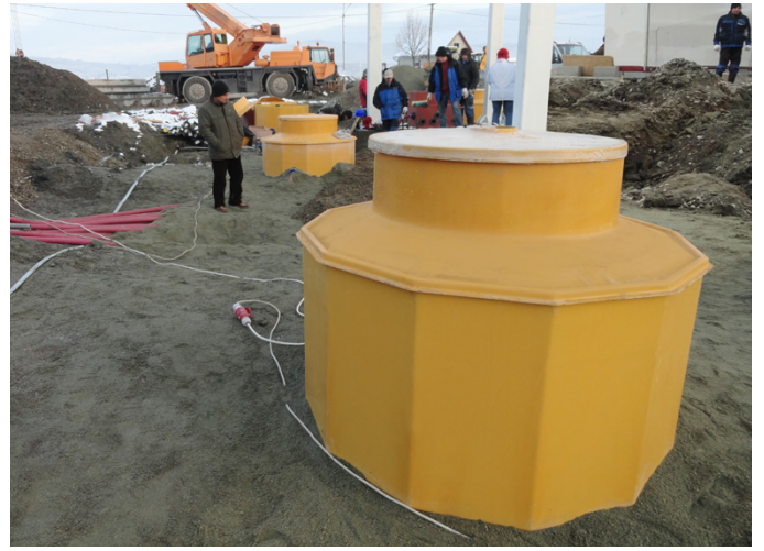
Gazprom have specified Fibrelite's fully conductive 1.6m dia chambers (S16) to facilitate easy maintenance post installation
