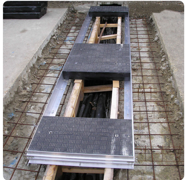
Fibrelite composite trench covers and aluminium frame during installation
