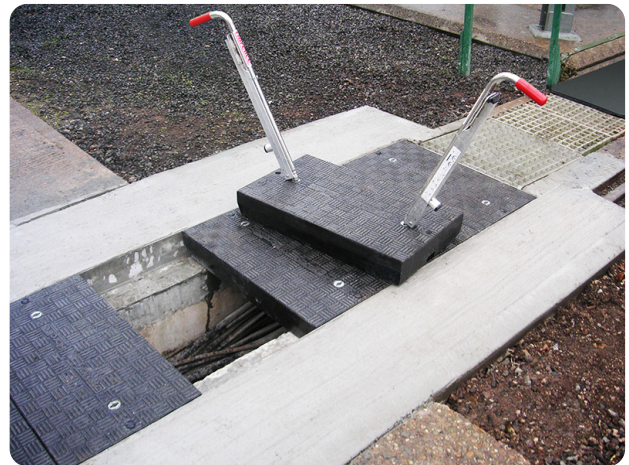
The Fibrelite lifting handles are specifically designed for operator use at the optimum ergonomic lifting range
